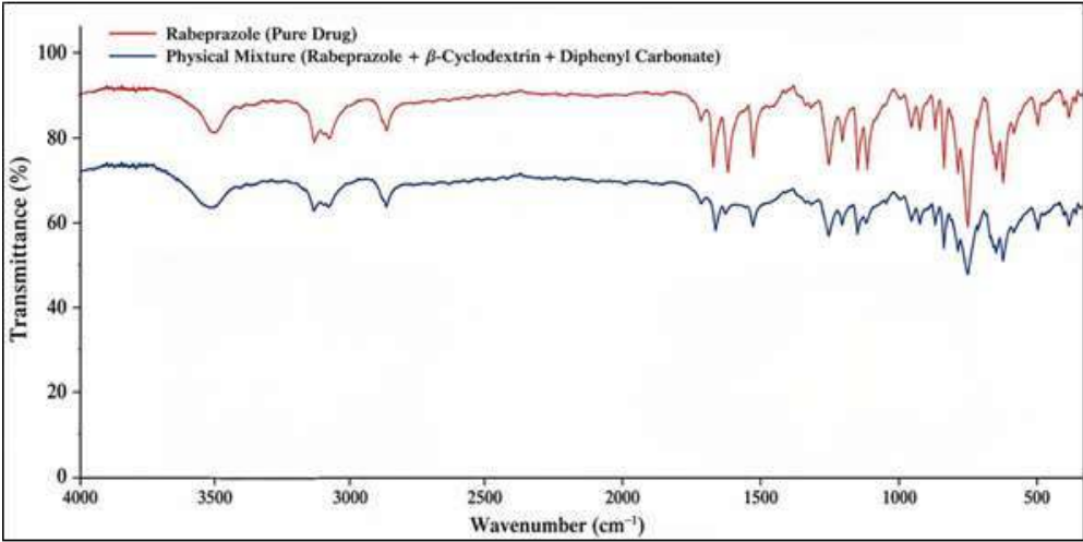
Figure 7: FTIR spectrum of rabeprazole-excipient physical mixture
