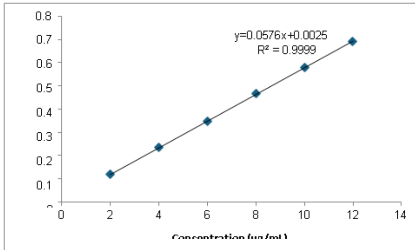
Figure 6: Calibration curve of rabeprazole at 283nm
