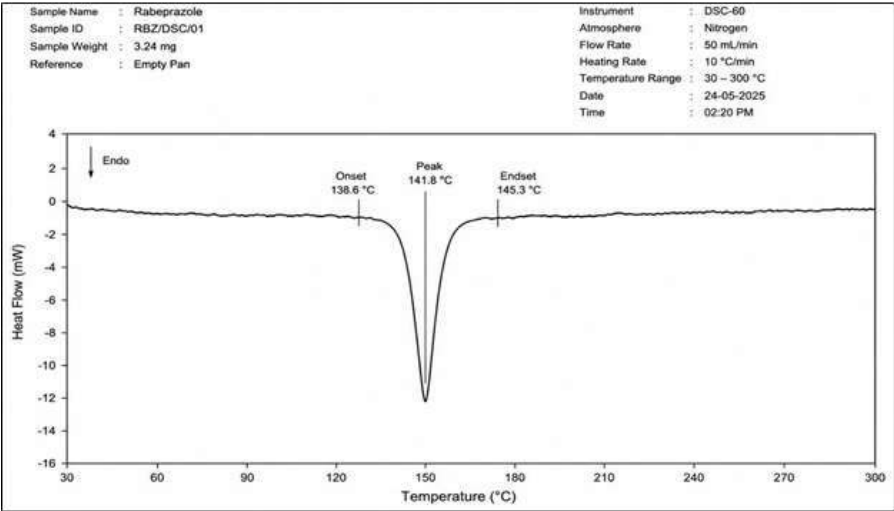
Figure 2: DSC thermogram of extracted rabeprazole
