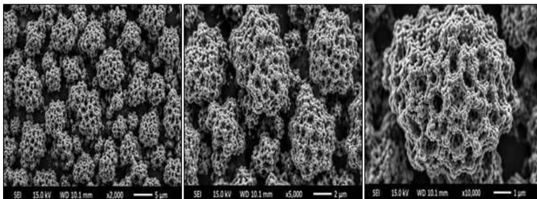
Figure 12: SEM micrographs of the optimized rabeprazole-loaded \beta -cyclodextrin nanosponge formulation (F5)
