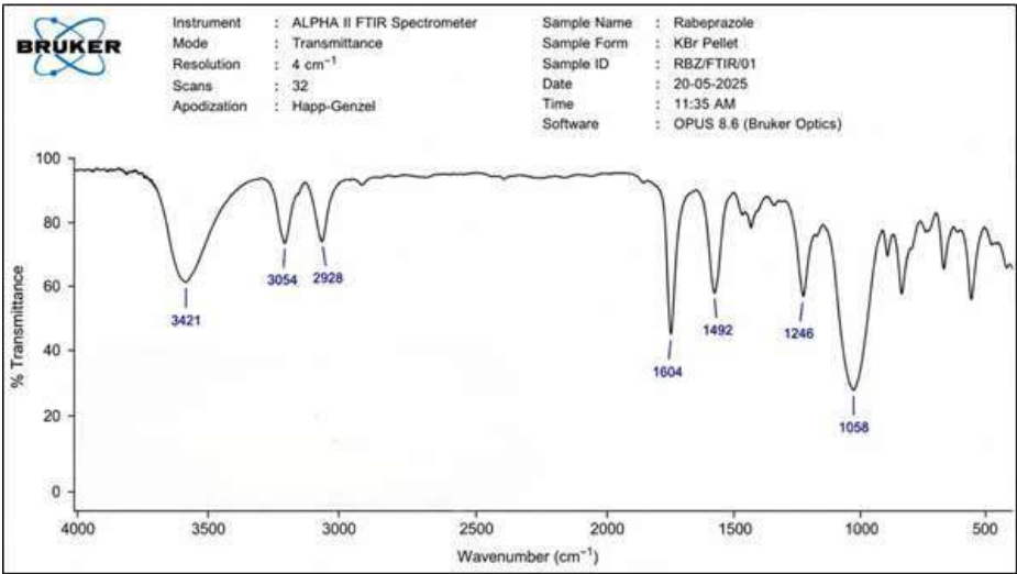
Figure 1: FTIR spectrum of extracted rabeprazole
