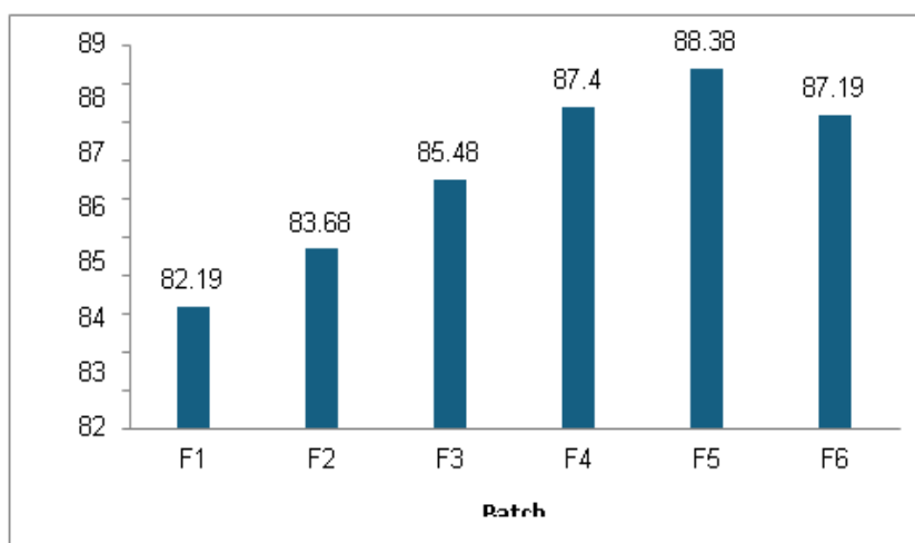
Figure 15: Production yield of rabeprazole-loaded \beta -cyclodextrin nanosponge formulations
