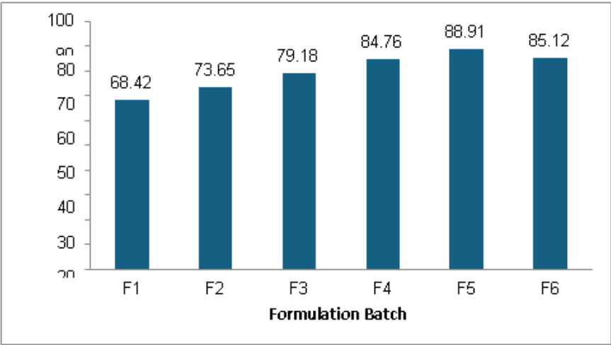
Figure 13: Entrapment efficiency of rabeprazole-loaded β-cyclodextrin nanosponge formulations
