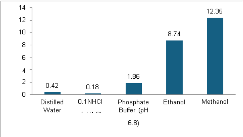
Figure 3: Solubility profile of extracted rabeprazole in different media
