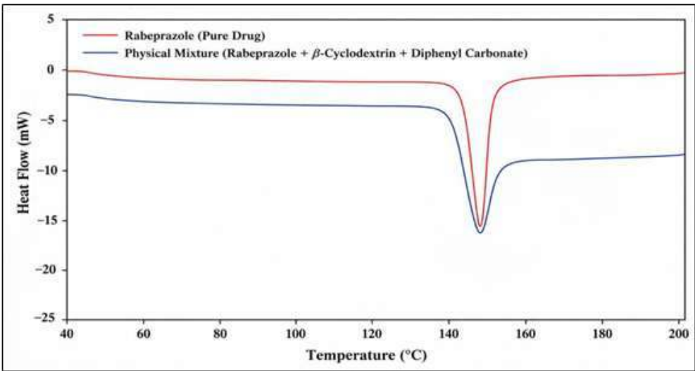
Figure 8: DSC thermogram of rabeprazole-excipient physical mixture
