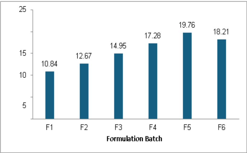
Figure 14: Drug loading capacity of rabeprazole-loaded β-cyclodextrin nanosponge formulations
