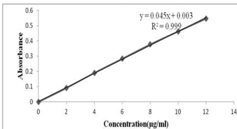
Figure 1: Calibration curve of Atorvastatin calcium in methanol
