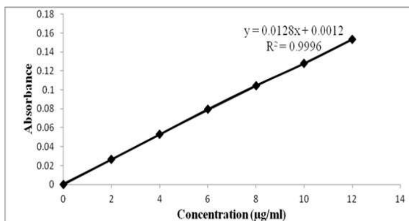
Figure 2: Calibration curve of Atorvastatin calcium in phosphate buffer pH 6.8
