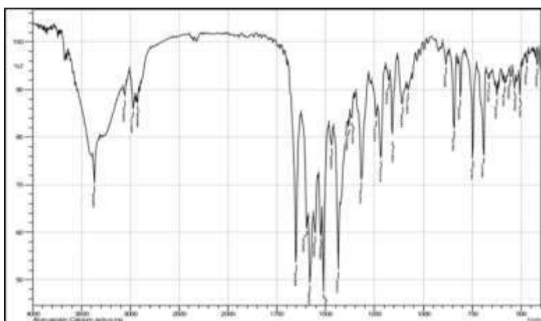
Figure 4: IR Spectroscopy of Atorvastatin calcium
