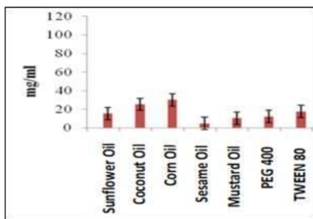
Figure 3: Solubility profile of Atorvastatin calcium
