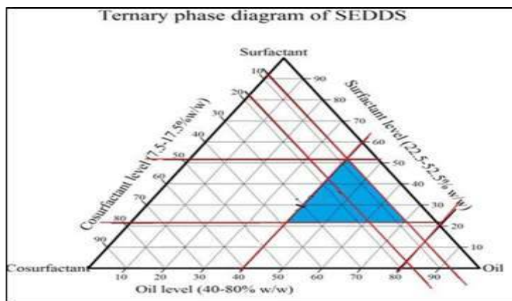
Figure5: Ternary phase diagram of Atorvastatin calcium SEDDS
